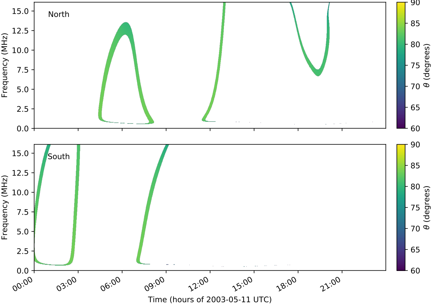
expres_cassini_jupiter_ganymede_isaac_lossc-wid1deg_3kev_20030511_v01.cdf
