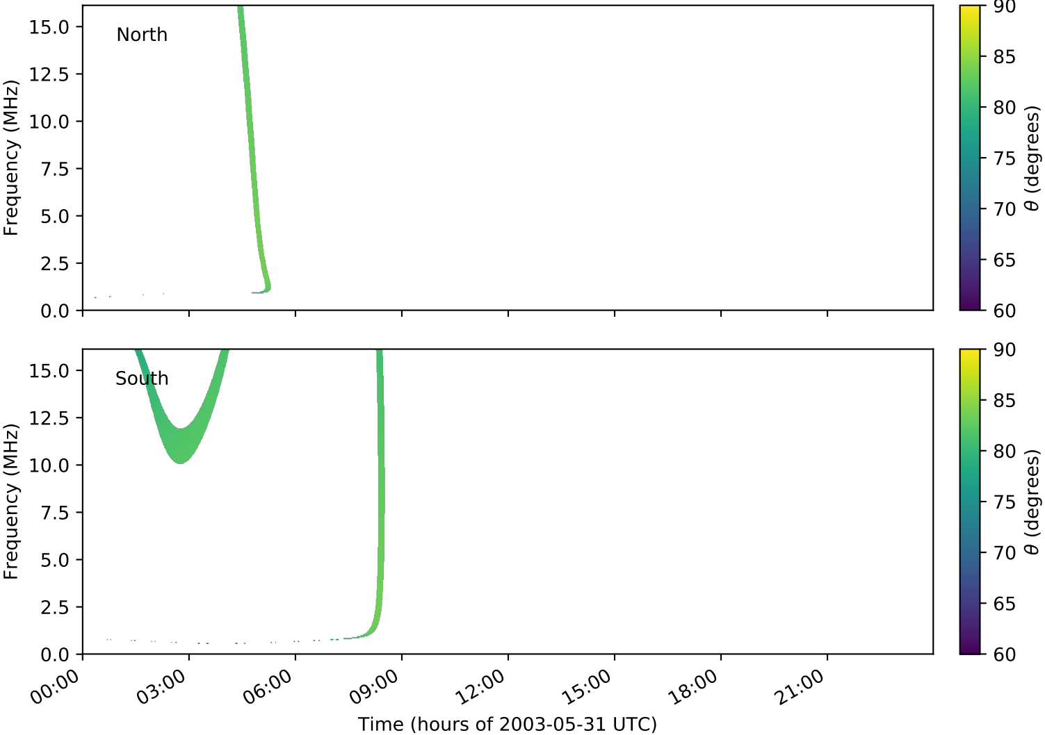
expres_cassini_jupiter_europa_isaac_lossc-wid1deg_3kev_20030531_v01.cdf
