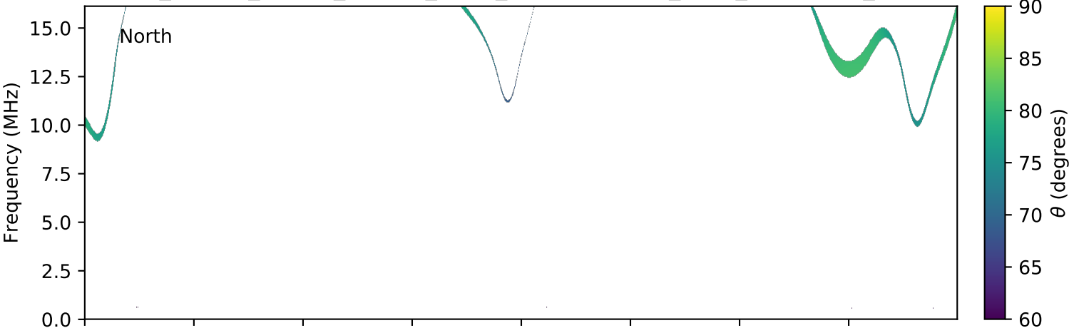
expres_cassini_jupiter_europa_isaac_lossc-wid1deg_3kev_20030530_v01.cdf
