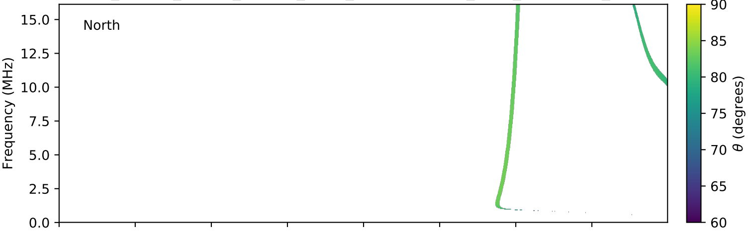
expres_cassini_jupiter_europa_isaac_lossc-wid1deg_3kev_20030529_v01.cdf
