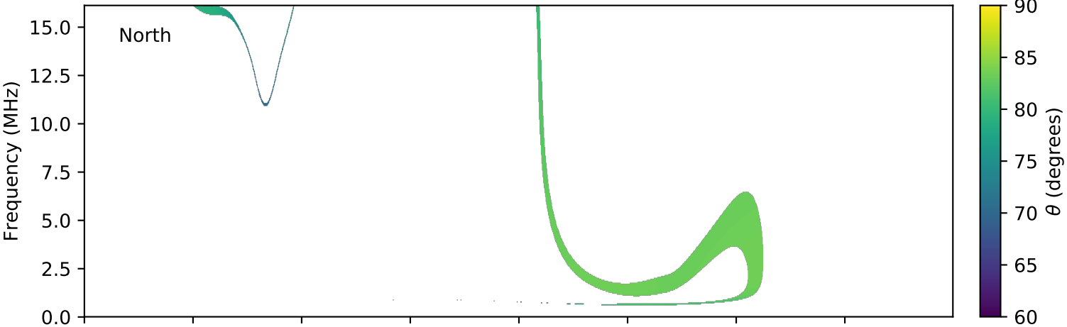
expres_cassini_jupiter_europa_isaac_lossc-wid1deg_3kev_20030527_v01.cdf
