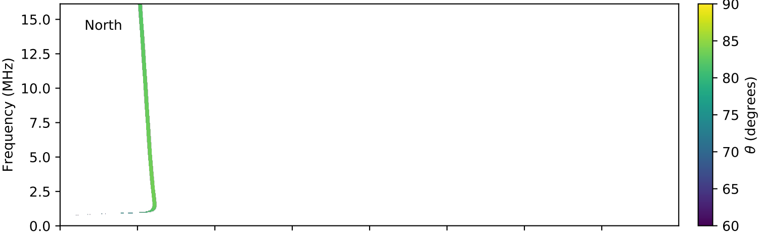
expres_cassini_jupiter_europa_isaac_lossc-wid1deg_3kev_20030524_v01.cdf
