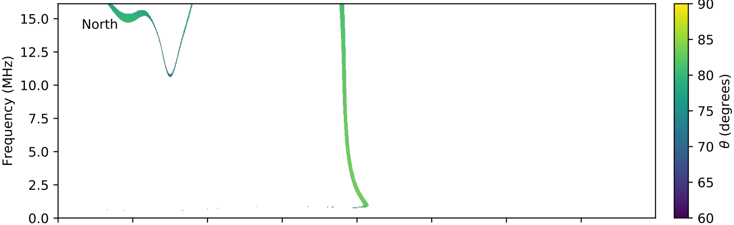
expres_cassini_jupiter_europa_isaac_lossc-wid1deg_3kev_20030520_v01.cdf
