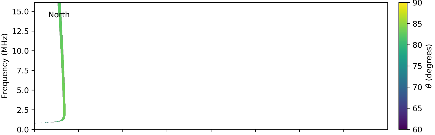
expres_cassini_jupiter_europa_isaac_lossc-wid1deg_3kev_20030517_v01.cdf
