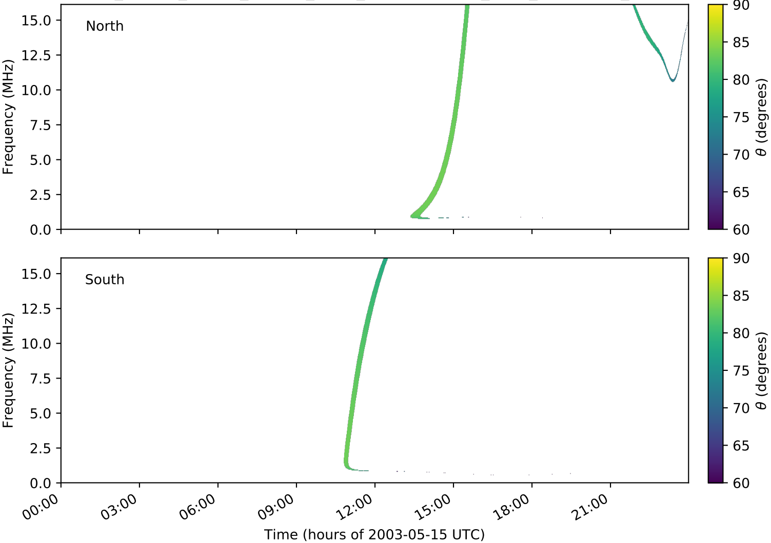
expres_cassini_jupiter_europa_isaac_lossc-wid1deg_3kev_20030515_v01.cdf
