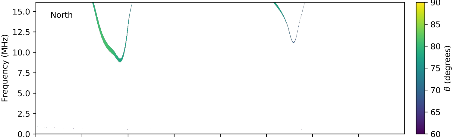
expres_cassini_jupiter_europa_isaac_lossc-wid1deg_3kev_20030512_v01.cdf
