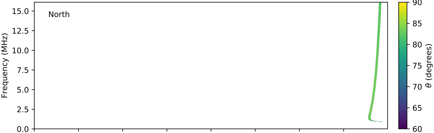
expres_cassini_jupiter_europa_isaac_lossc-wid1deg_3kev_20030511_v01.cdf
