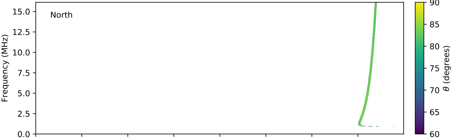
expres_cassini_jupiter_europa_isaac_lossc-wid1deg_3kev_20030504_v01.cdf
