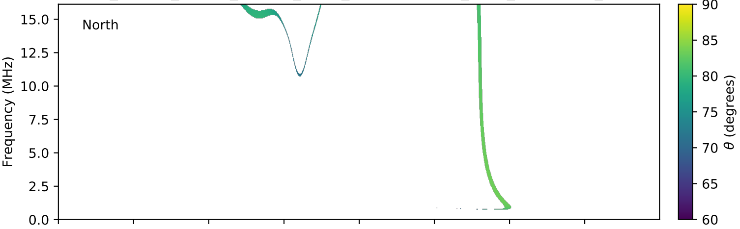
expres_cassini_jupiter_europa_isaac_lossc-wid1deg_3kev_20030502_v01.cdf
