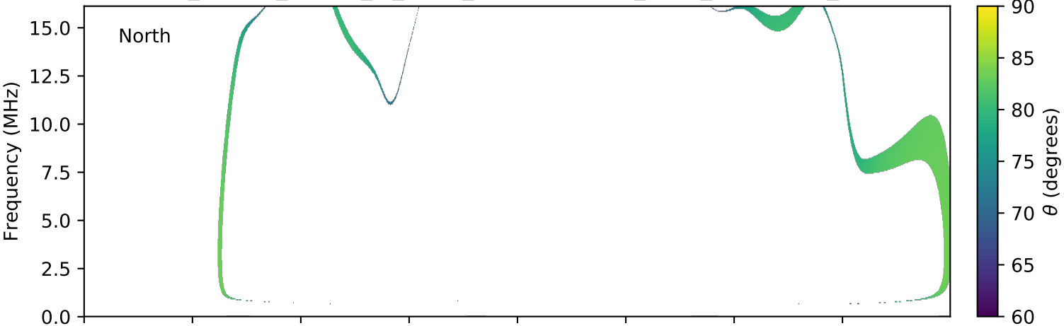
expres_cassini_jupiter_io_isaac_lossc-wid1deg_3kev_20030427_v01.cdf
