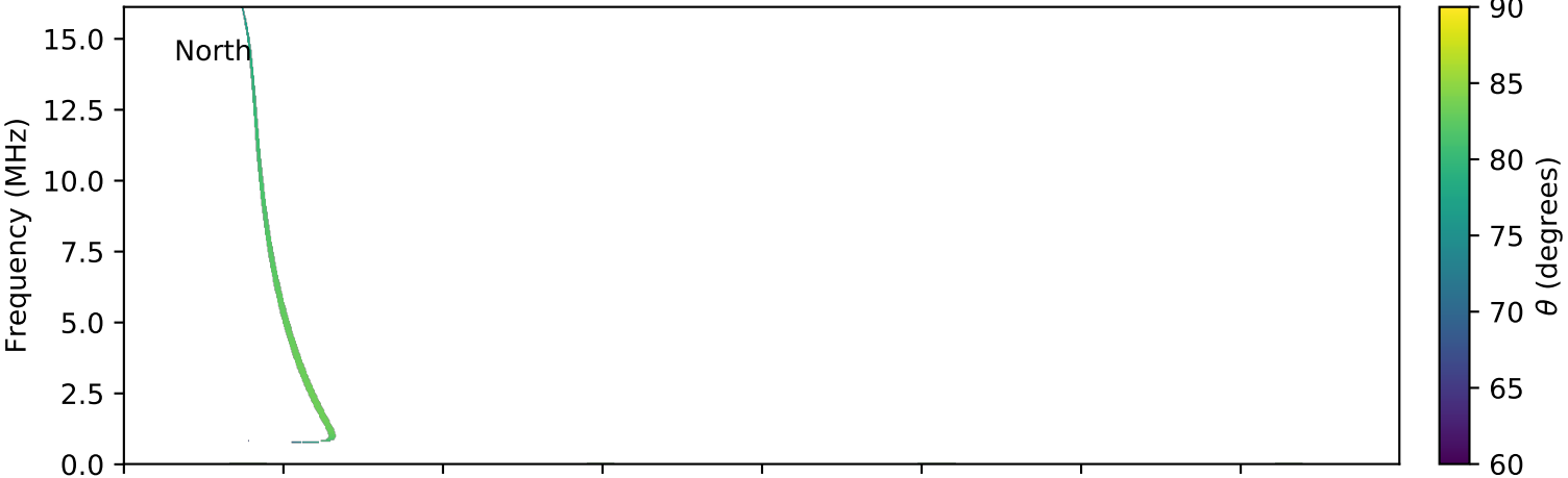
expres_cassini_jupiter_io_isaac_lossc-wid1deg_3kev_20030426_v01.cdf
