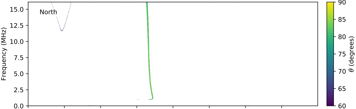
expres_cassini_jupiter_io_isaac_lossc-wid1deg_3kev_20030424_v01.cdf
