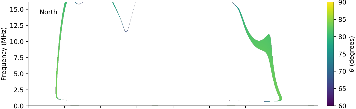
expres_cassini_jupiter_io_isaac_lossc-wid1deg_3kev_20030420_v01.cdf
