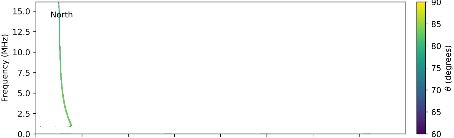
expres_cassini_jupiter_io_isaac_lossc-wid1deg_3kev_20030419_v01.cdf
