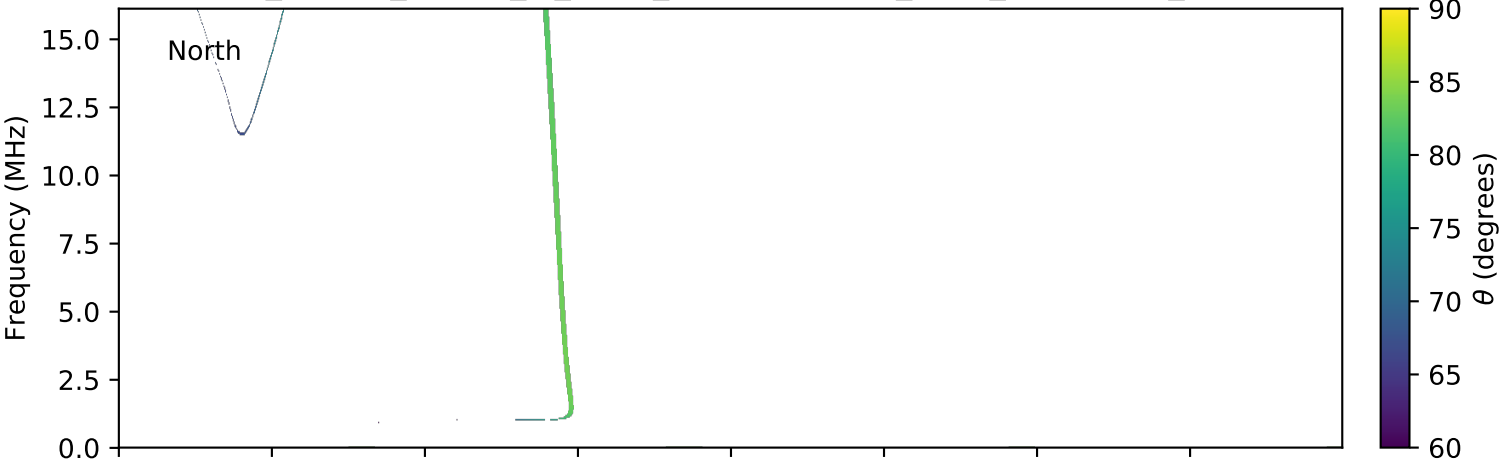
expres_cassini_jupiter_io_isaac_lossc-wid1deg_3kev_20030417_v01.cdf
