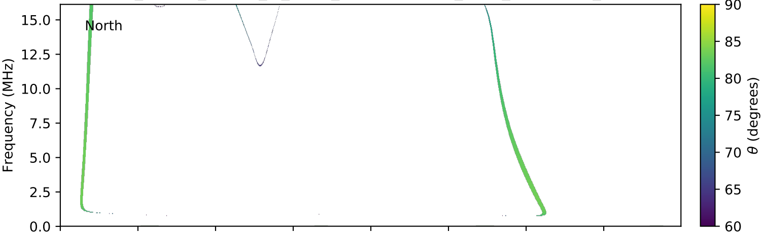
expres_cassini_jupiter_io_isaac_lossc-wid1deg_3kev_20030413_v01.cdf
