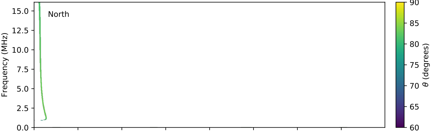
expres_cassini_jupiter_io_isaac_lossc-wid1deg_3kev_20030412_v01.cdf
