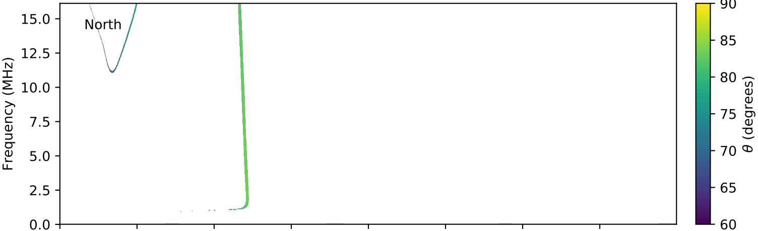
expres_cassini_jupiter_io_isaac_lossc-wid1deg_3kev_20030410_v01.cdf
