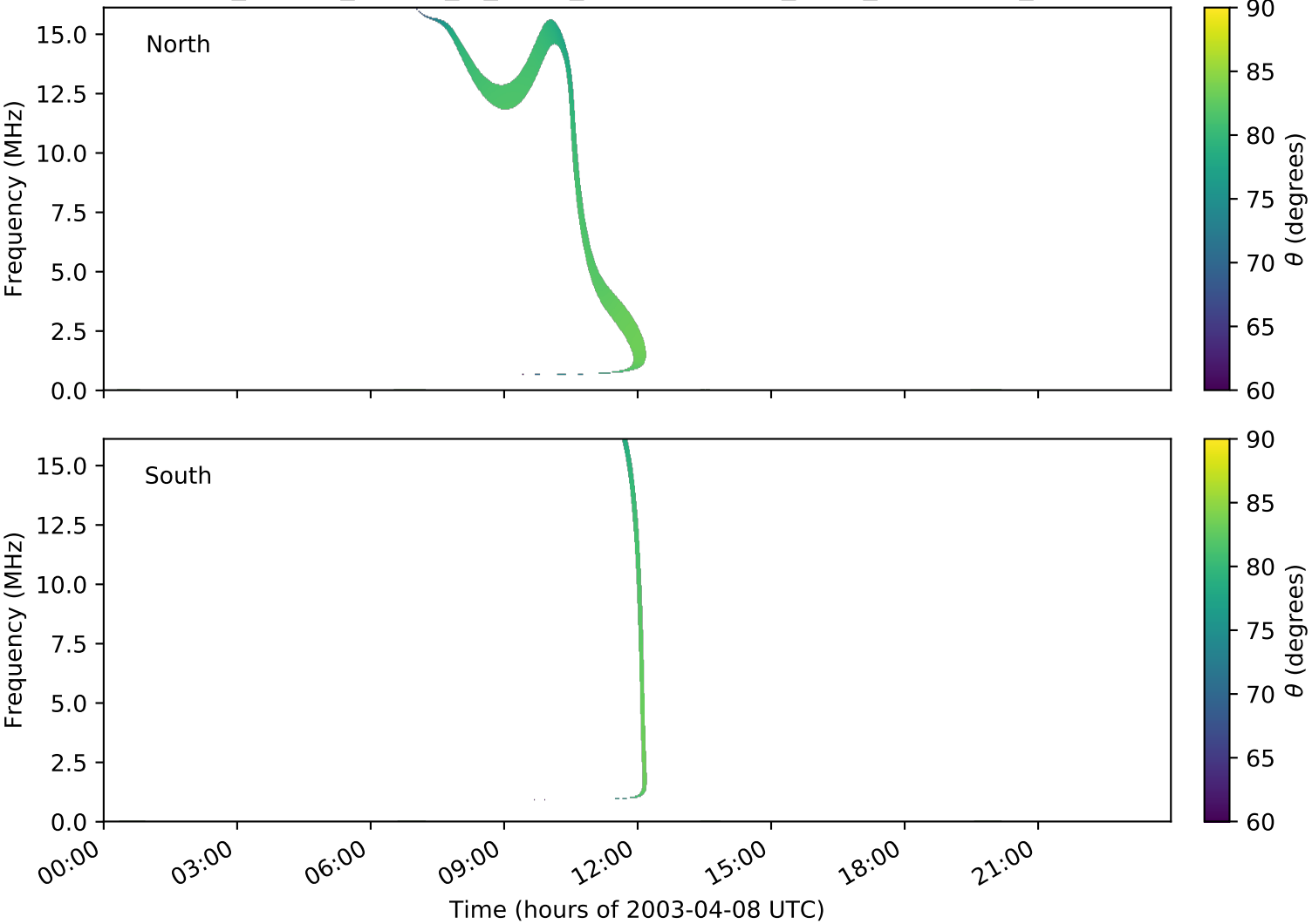
expres_cassini_jupiter_io_isaac_lossc-wid1deg_3kev_20030408_v01.cdf
