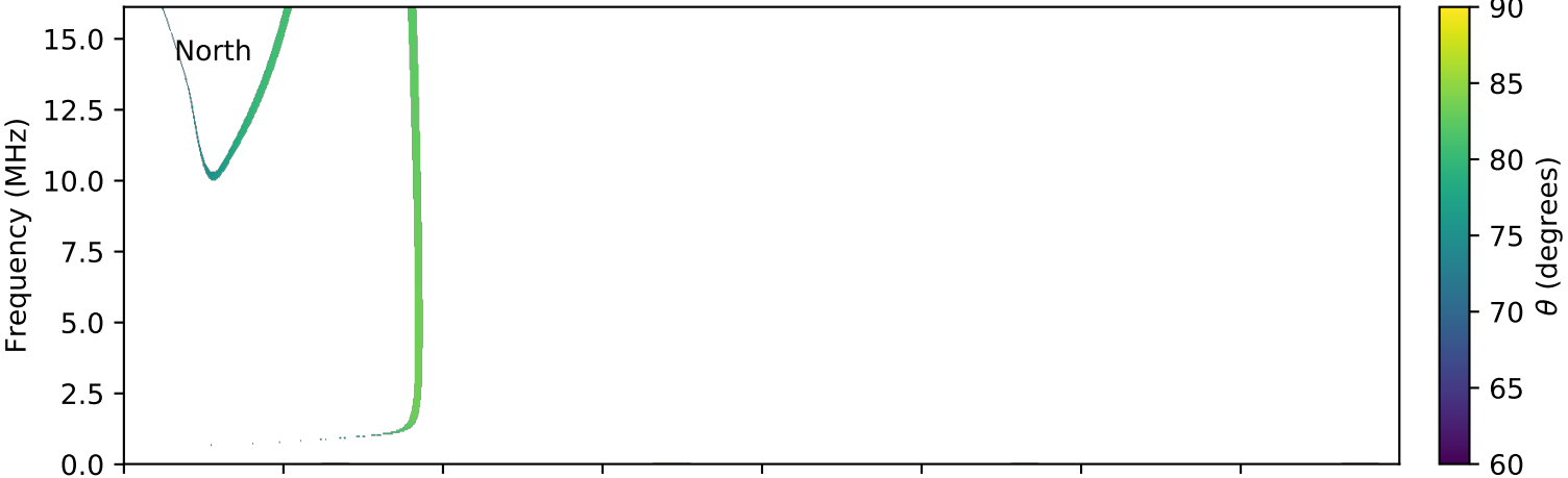
expres_cassini_jupiter_io_isaac_lossc-wid1deg_3kev_20030403_v01.cdf
