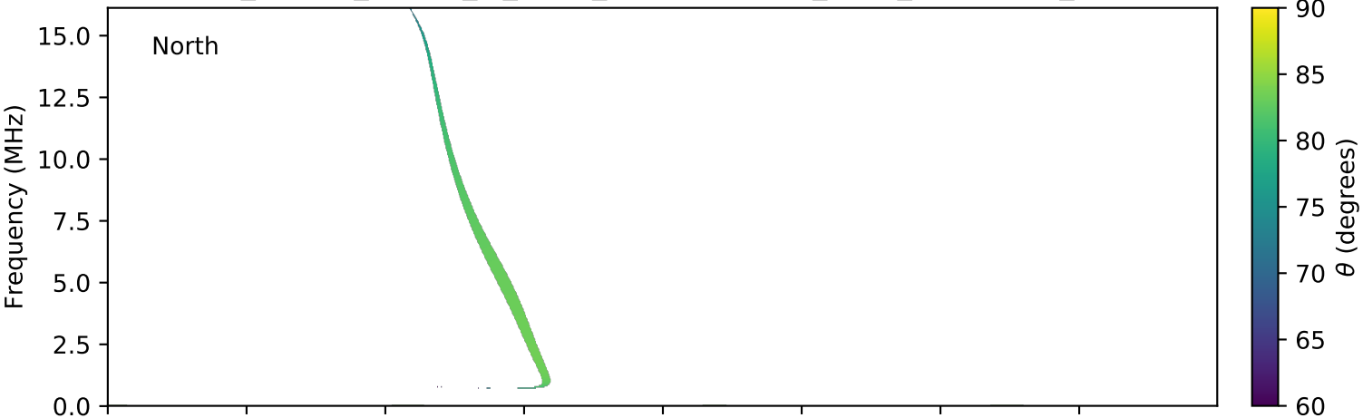
expres_cassini_jupiter_io_isaac_lossc-wid1deg_3kev_20030401_v01.cdf
