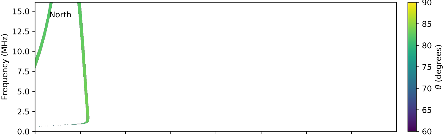
expres_cassini_jupiter_ganymede_isaac_lossc-wid1deg_3kev_20030430_v01.cdf
