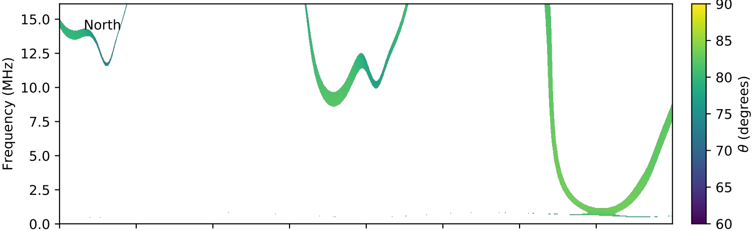
expres_cassini_jupiter_ganymede_isaac_lossc-wid1deg_3kev_20030429_v01.cdf
