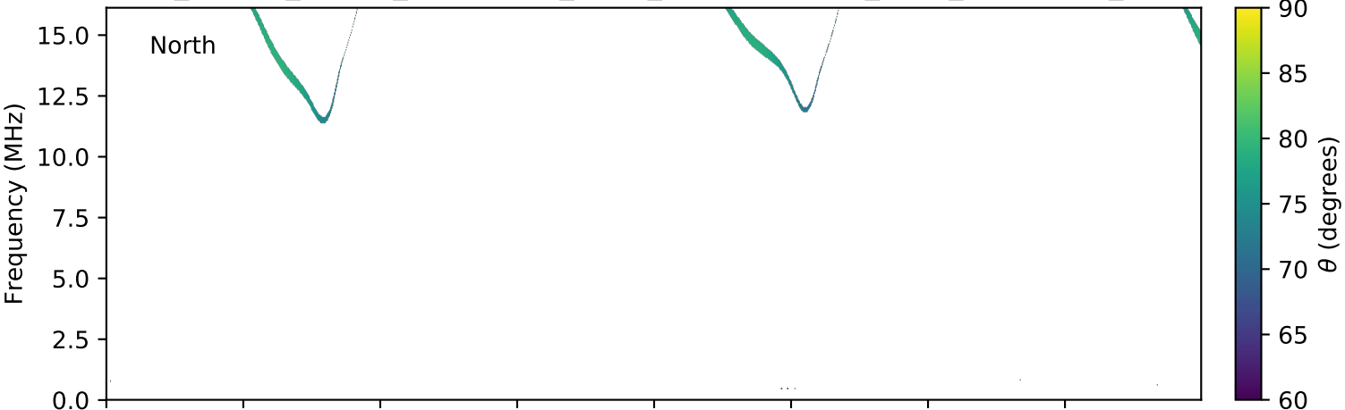
expres_cassini_jupiter_ganymede_isaac_lossc-wid1deg_3kev_20030428_v01.cdf
