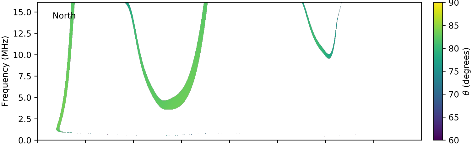
expres_cassini_jupiter_ganymede_isaac_lossc-wid1deg_3kev_20030427_v01.cdf
