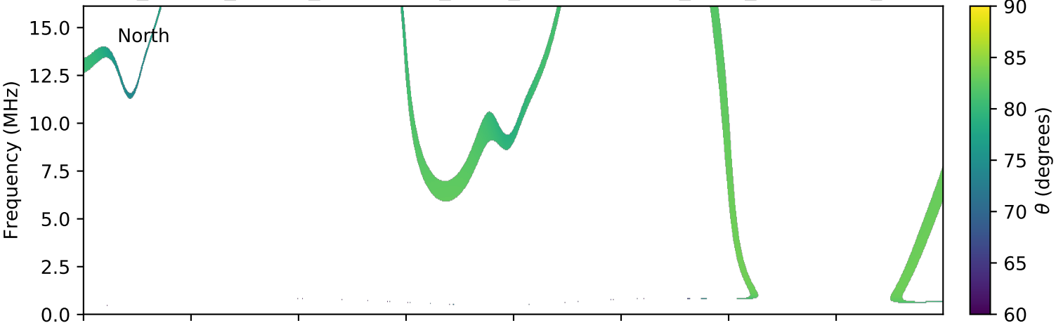
expres_cassini_jupiter_ganymede_isaac_lossc-wid1deg_3kev_20030422_v01.cdf
