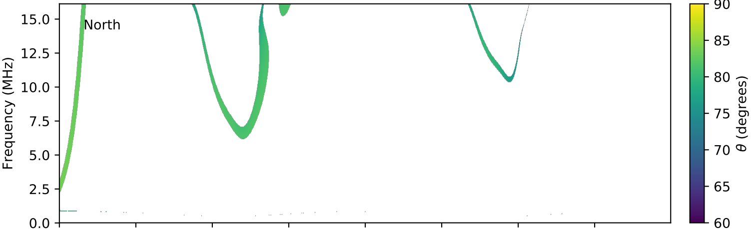
expres_cassini_jupiter_ganymede_isaac_lossc-wid1deg_3kev_20030420_v01.cdf
