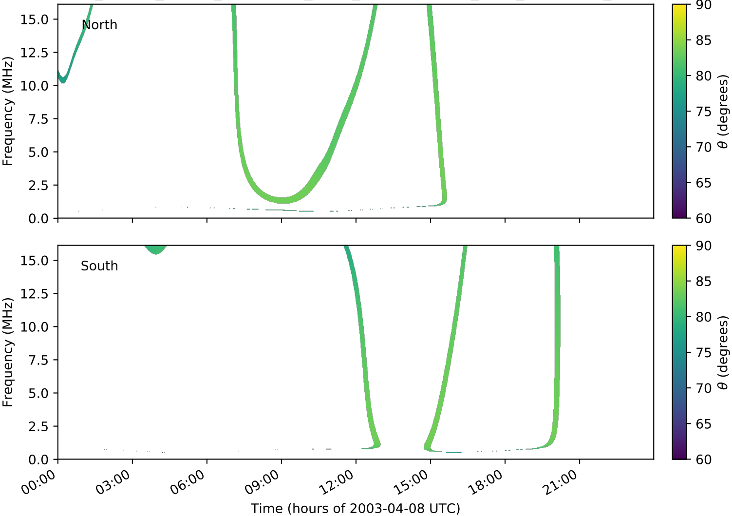
expres_cassini_jupiter_ganymede_isaac_lossc-wid1deg_3kev_20030408_v01.cdf
