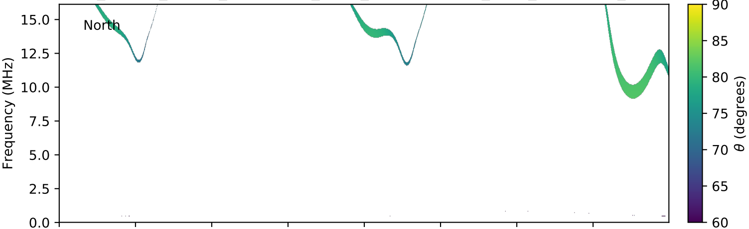
expres_cassini_jupiter_ganymede_isaac_lossc-wid1deg_3kev_20030407_v01.cdf
