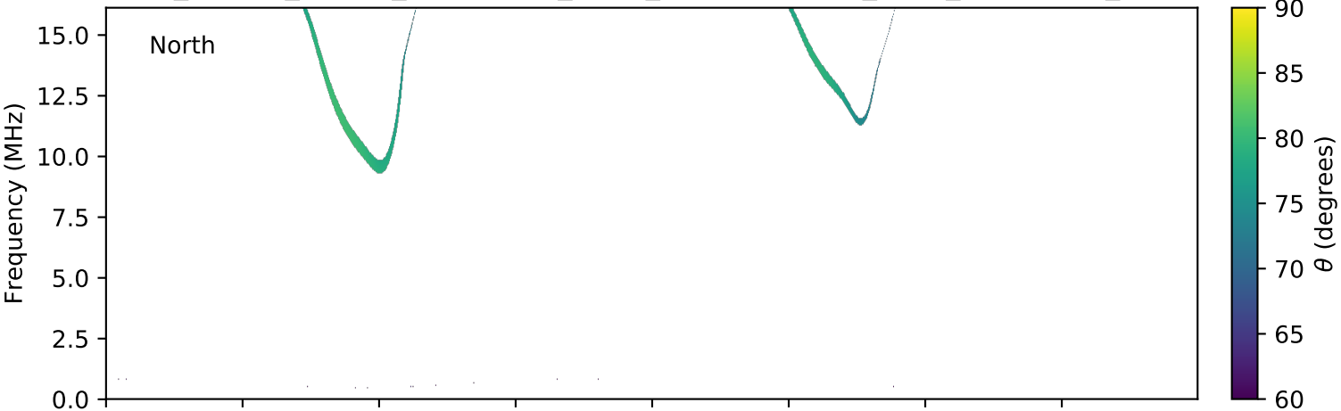
expres_cassini_jupiter_ganymede_isaac_lossc-wid1deg_3kev_20030406_v01.cdf
