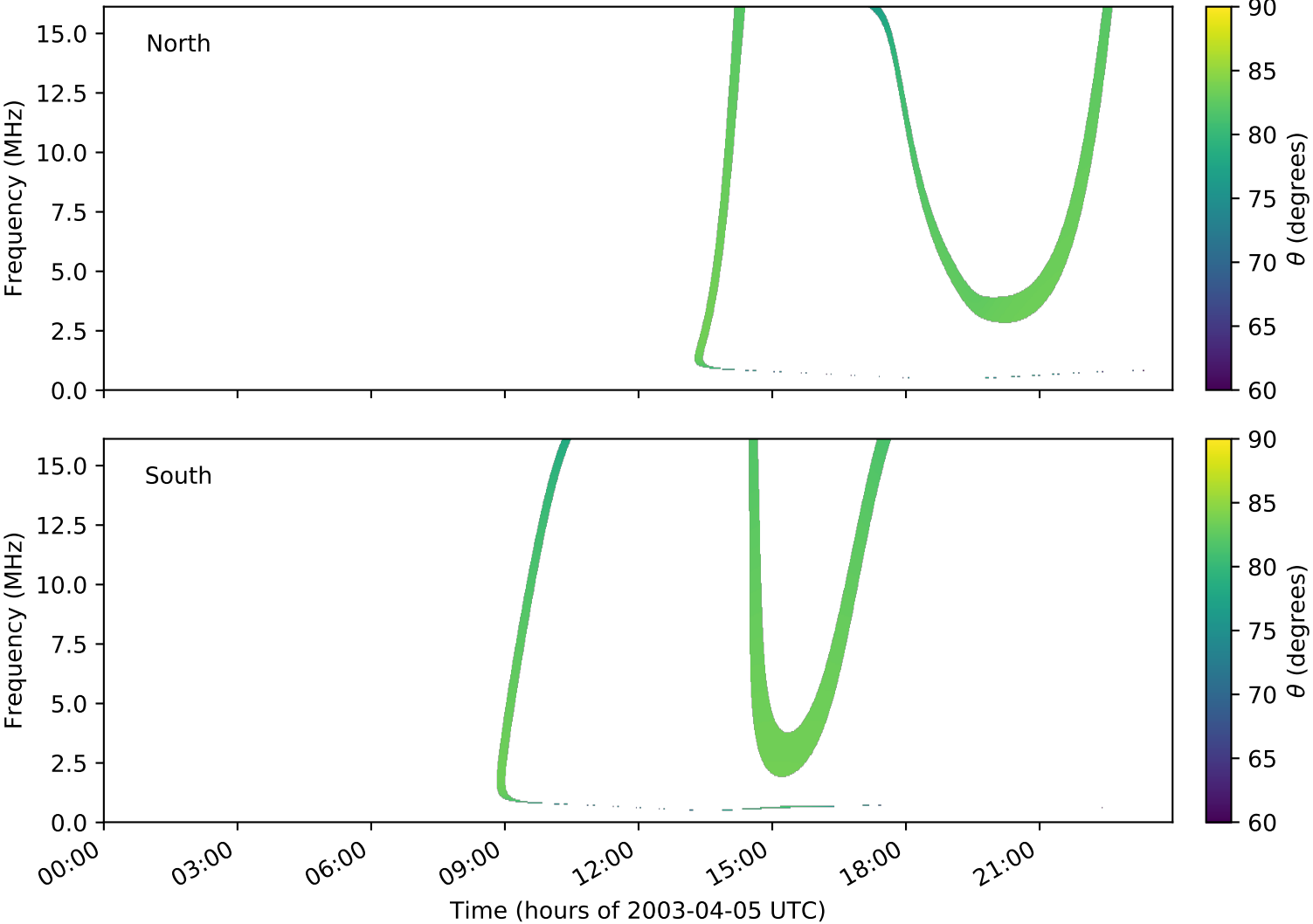
expres_cassini_jupiter_ganymede_isaac_lossc-wid1deg_3kev_20030405_v01.cdf
