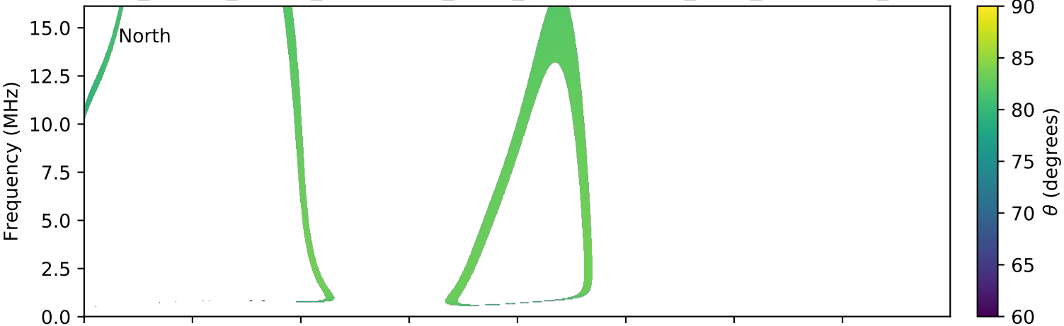
expres_cassini_jupiter_ganymede_isaac_lossc-wid1deg_3kev_20030401_v01.cdf
