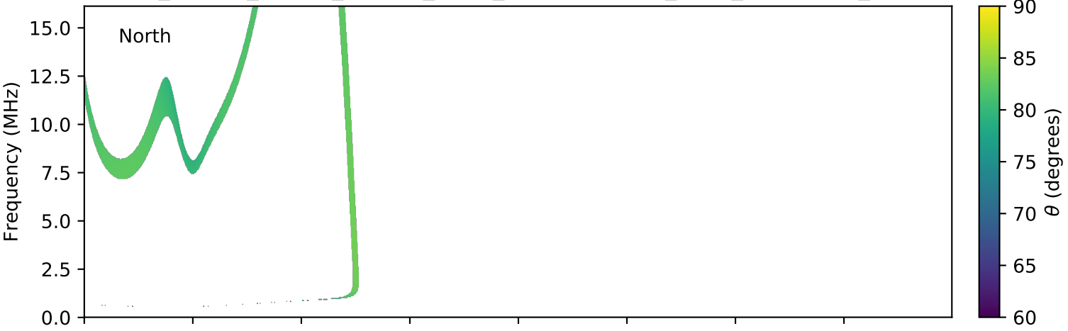
expres_cassini_jupiter_europa_isaac_lossc-wid1deg_3kev_20030429_v01.cdf
