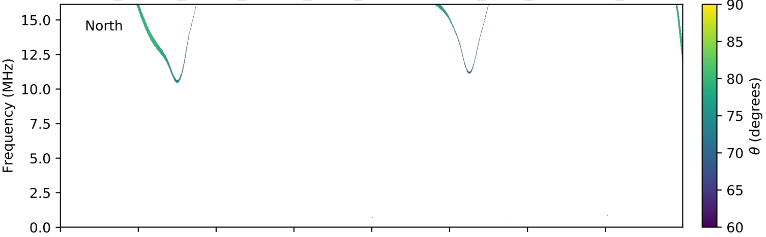
expres_cassini_jupiter_europa_isaac_lossc-wid1deg_3kev_20030428_v01.cdf
