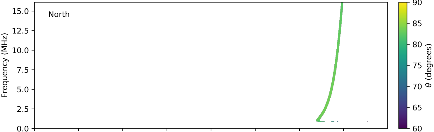
expres_cassini_jupiter_europa_isaac_lossc-wid1deg_3kev_20030427_v01.cdf
