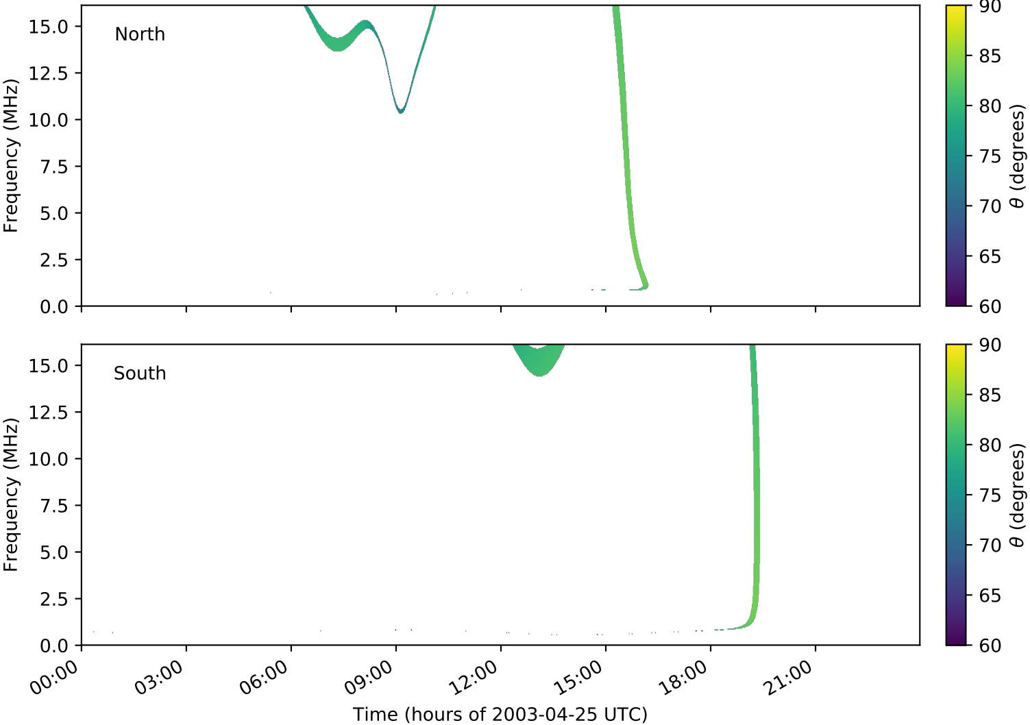
expres_cassini_jupiter_europa_isaac_lossc-wid1deg_3kev_20030425_v01.cdf
