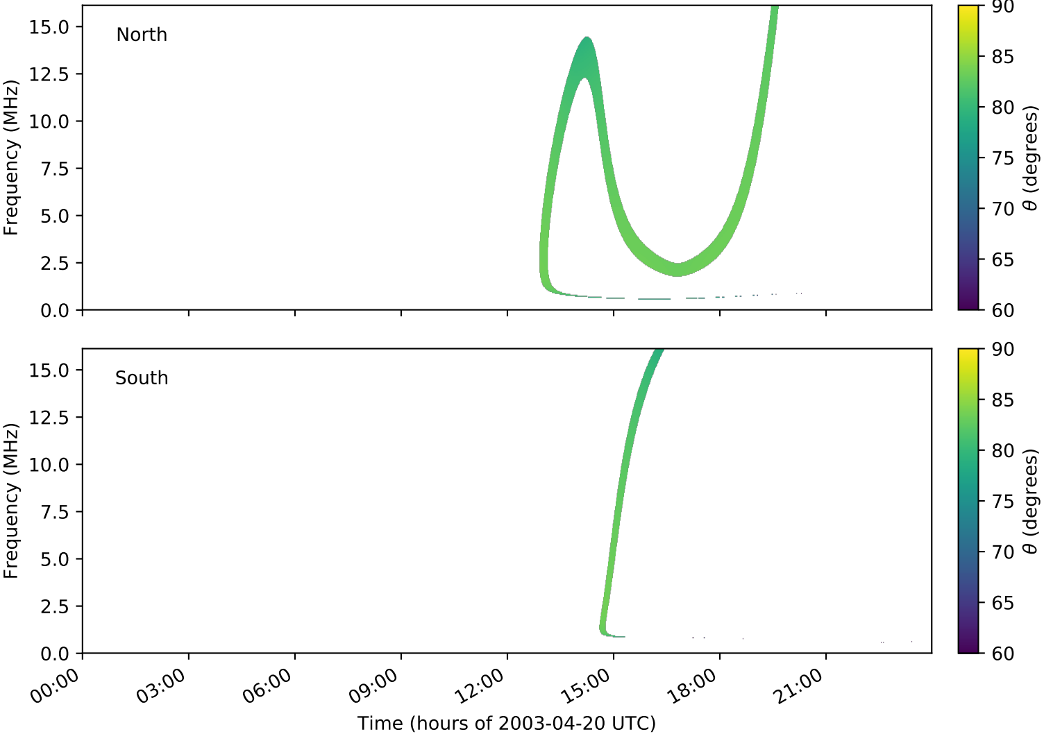
expres_cassini_jupiter_europa_isaac_lossc-wid1deg_3kev_20030420_v01.cdf
