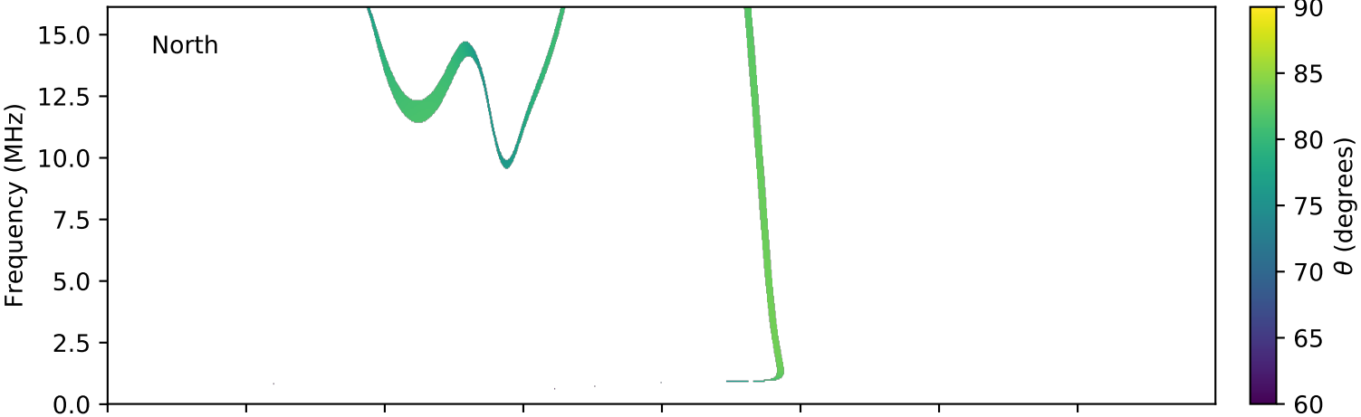
expres_cassini_jupiter_europa_isaac_lossc-wid1deg_3kev_20030418_v01.cdf
