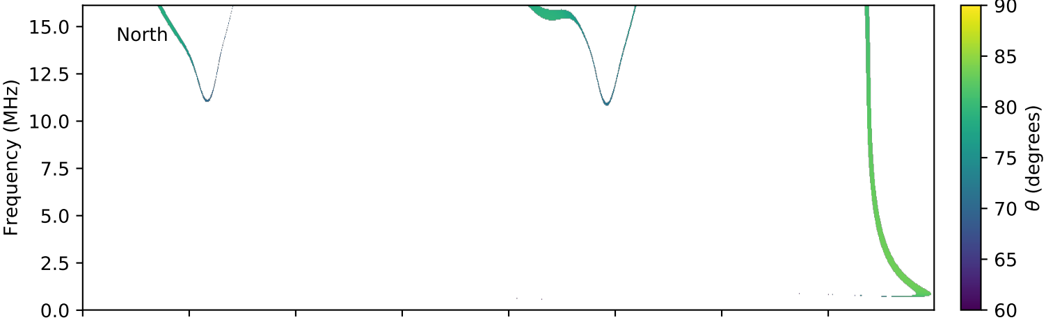
expres_cassini_jupiter_europa_isaac_lossc-wid1deg_3kev_20030414_v01.cdf
