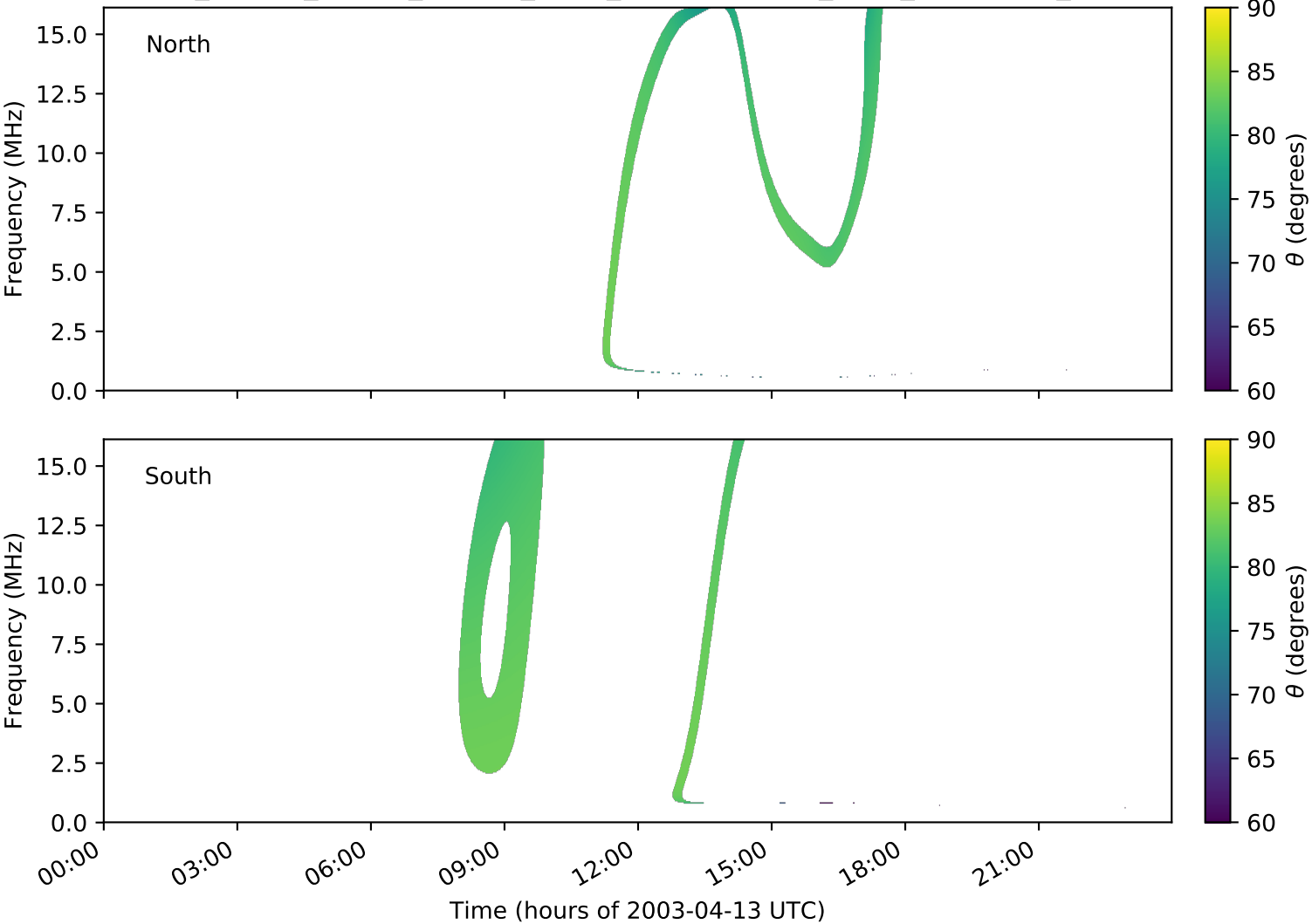
expres_cassini_jupiter_europa_isaac_lossc-wid1deg_3kev_20030413_v01.cdf
