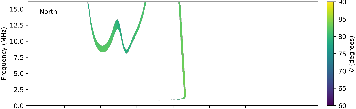
expres_cassini_jupiter_europa_isaac_lossc-wid1deg_3kev_20030411_v01.cdf
