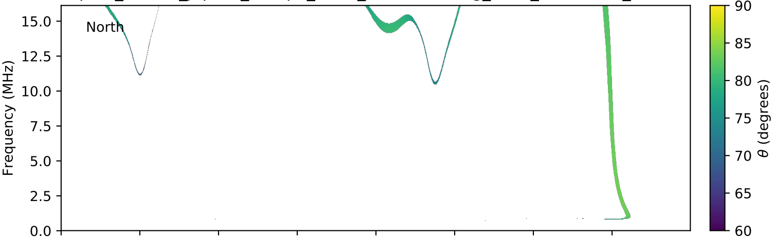
expres_cassini_jupiter_europa_isaac_lossc-wid1deg_3kev_20030407_v01.cdf
