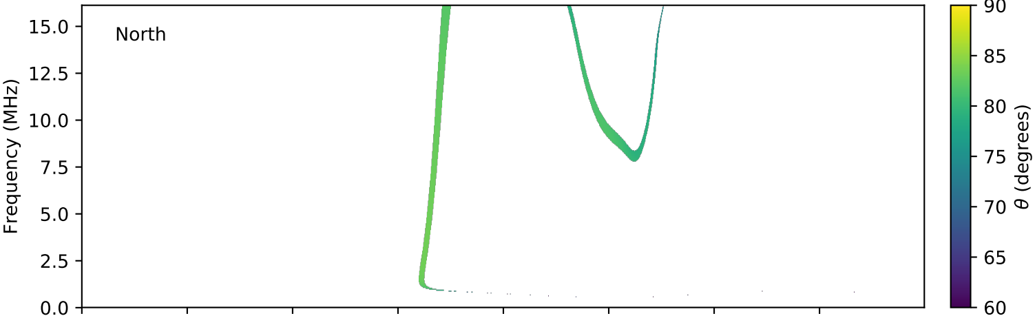
expres_cassini_jupiter_europa_isaac_lossc-wid1deg_3kev_20030406_v01.cdf
