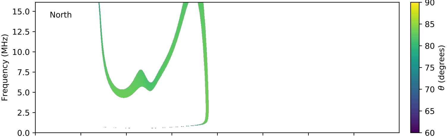
expres_cassini_jupiter_europa_isaac_lossc-wid1deg_3kev_20030404_v01.cdf
