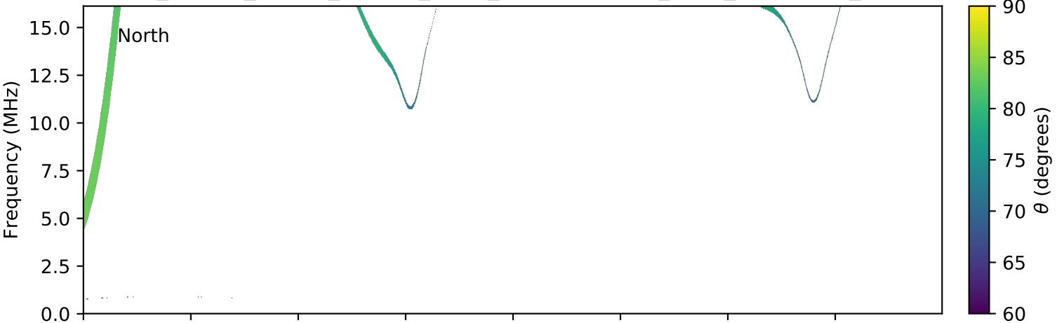
expres_cassini_jupiter_europa_isaac_lossc-wid1deg_3kev_20030403_v01.cdf
