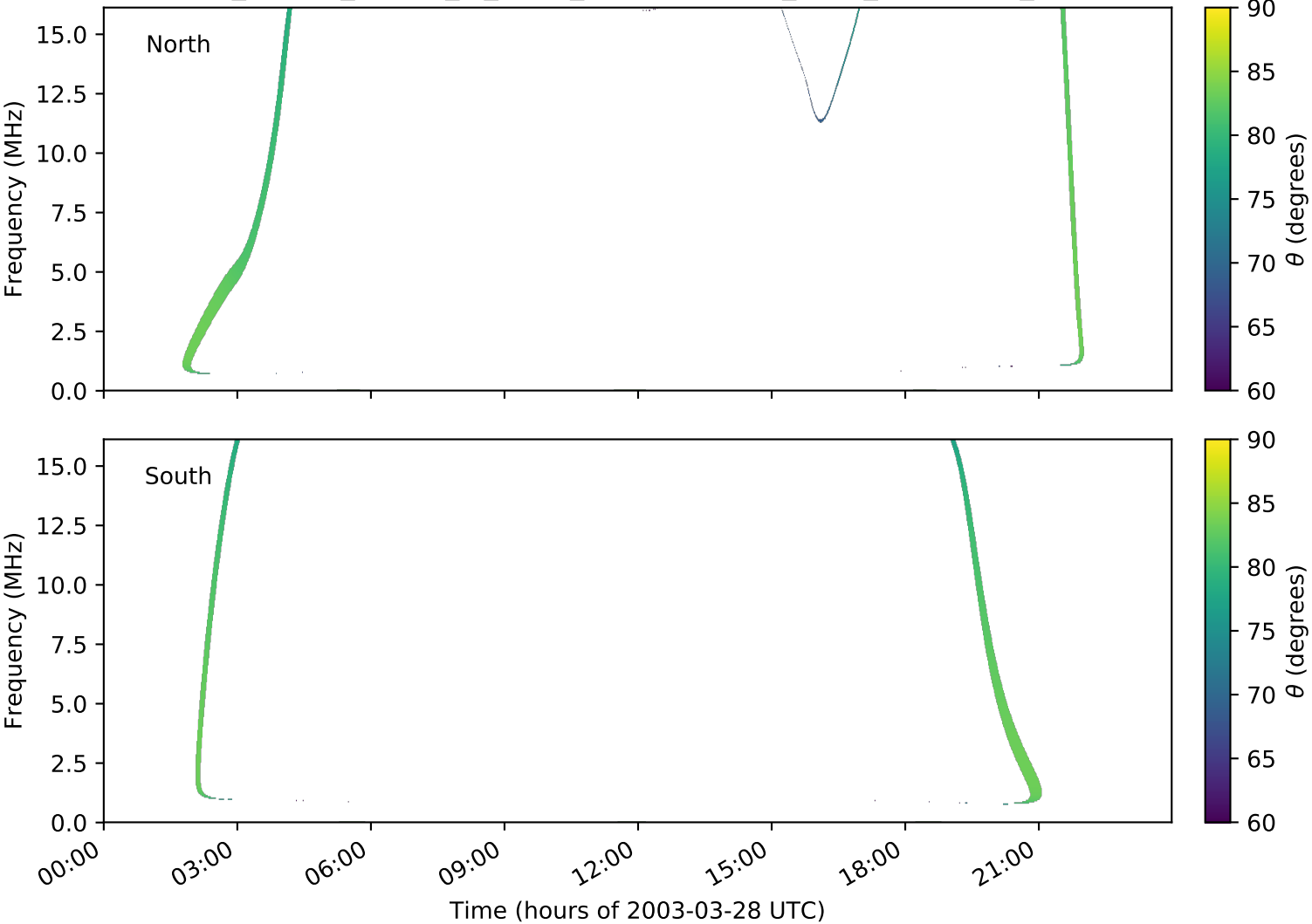
expres_cassini_jupiter_io_isaac_lossc-wid1deg_3kev_20030328_v01.cdf
